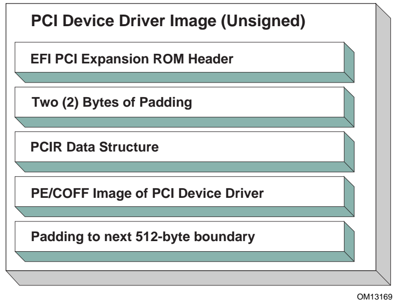
Figure 45. Unsigned PCI Driver Image Layout
