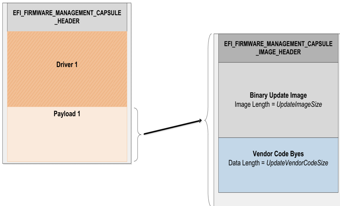
Figure 65. Firmware Management and Firmware Image Management headers
