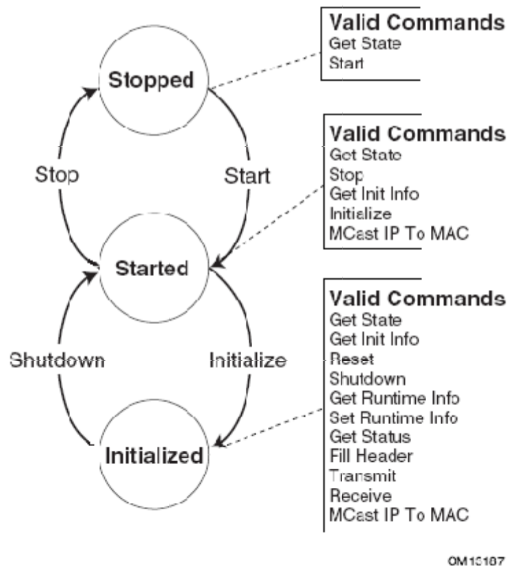
Figure 133. UNDI States, Transitions & Valid Commands
