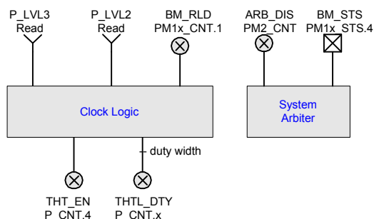
Figure 8-44 ACPI Clock Logic (One per Processor)
