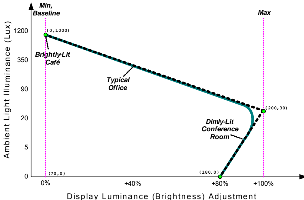
Figure 9-53 Example Response Curve for a Transflective Display
