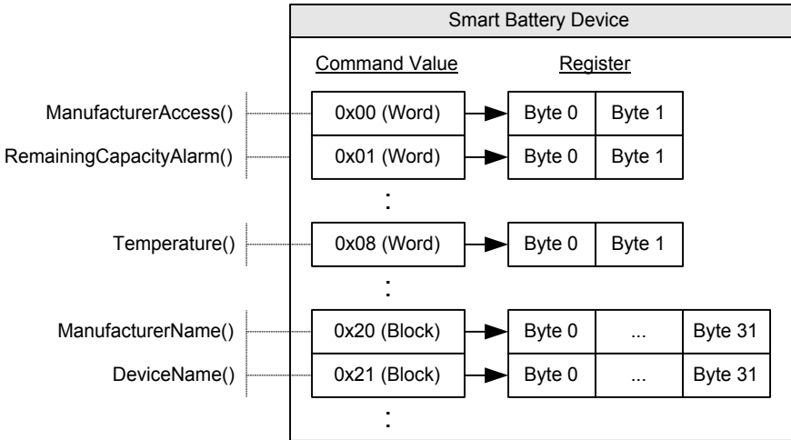
Figure 13-75 Smart Battery Device Virtual Registers
