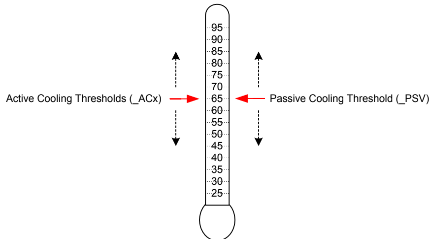
Figure 11-68 Active and Passive Threshold Values
