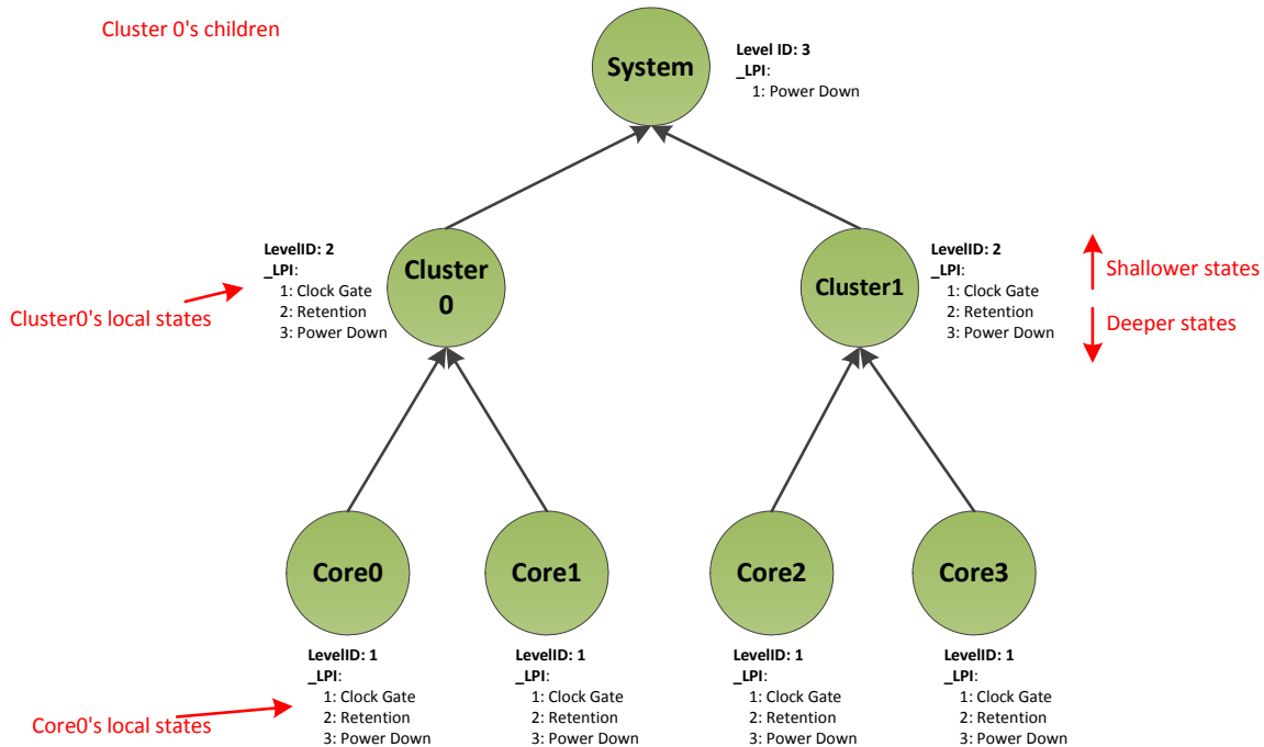
Figure 8-46 Power states for processor hierarchy
