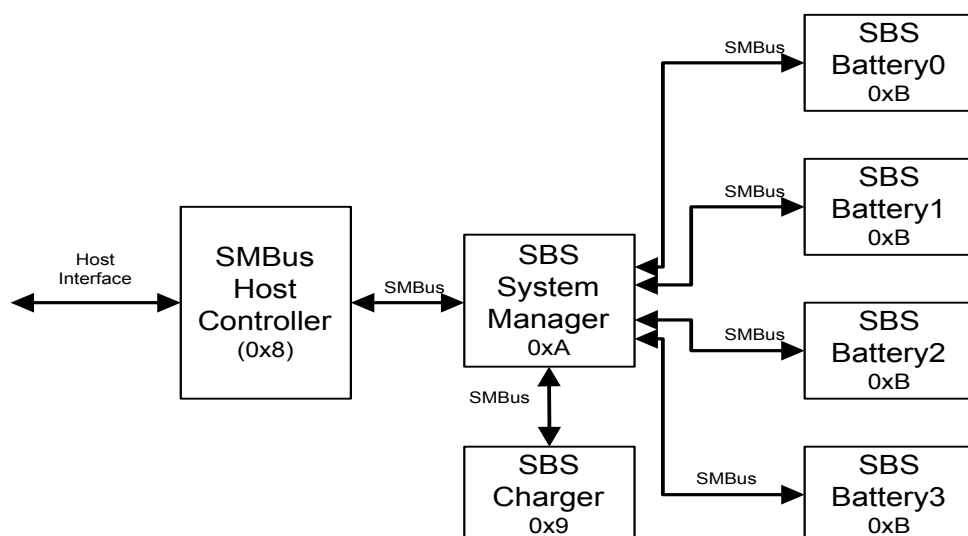
Figure 10-59 Typical Smart Battery Subsystem (SBS)
