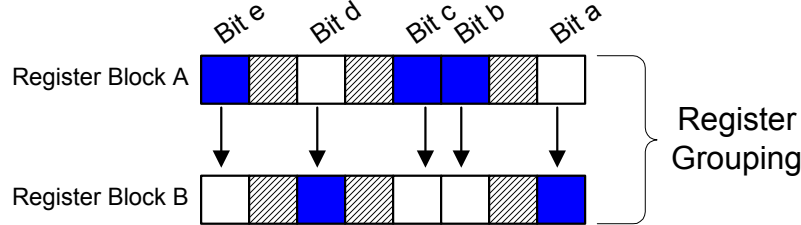
Figure 4-13 Example Fixed Hardware Feature Register Grouping
