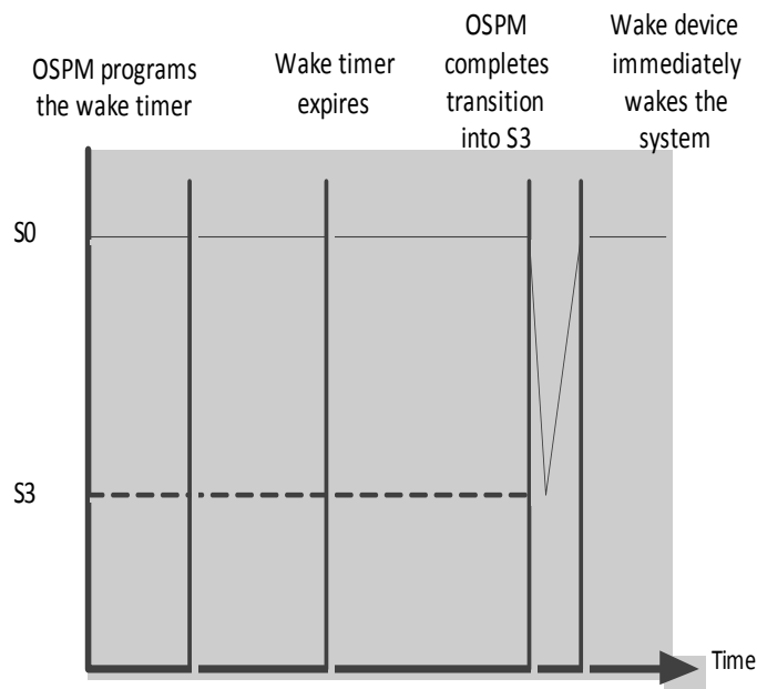
Figure 9-55 Persistence of expired timer events
