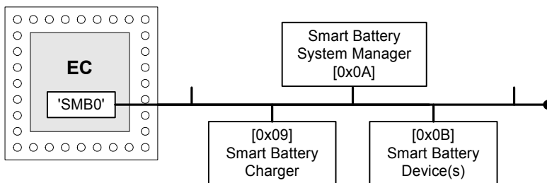
Figure 13-74 Smart Battery Subsystem Devices
