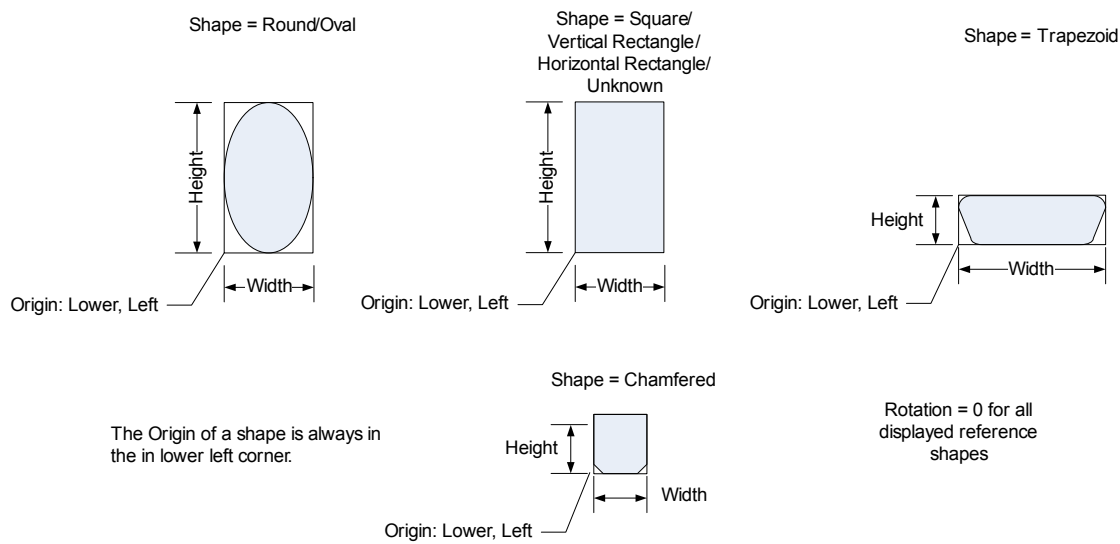
Figure 6-35 Default Shape Definitions
