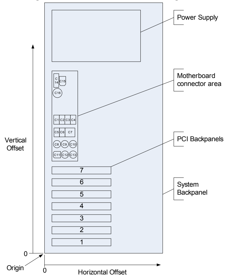
Figure 6-36 PLD Back Panel Rendering
