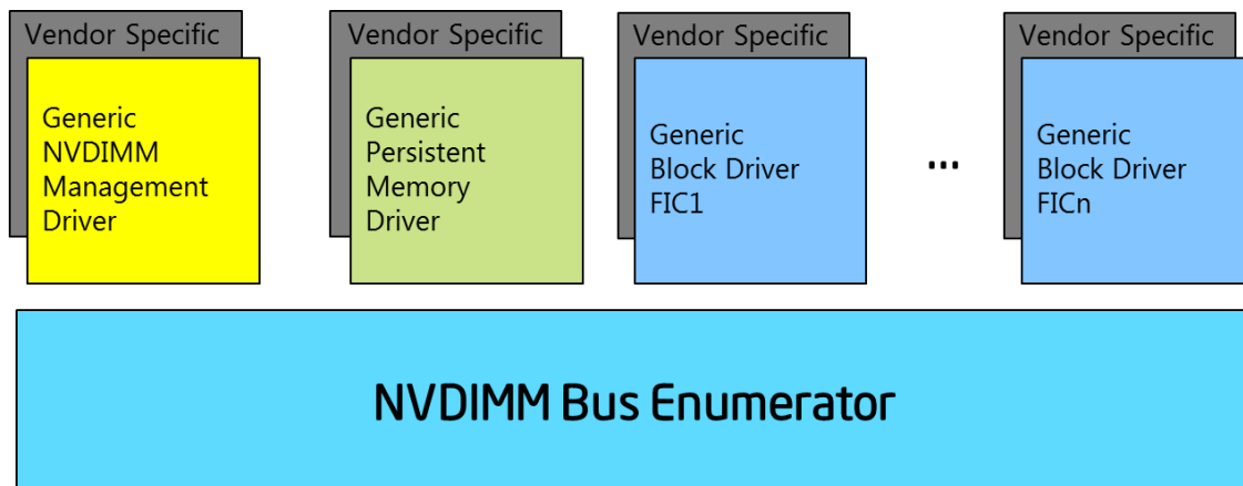
Figure 9-58 Vendor/Device Specific Driver Loading
