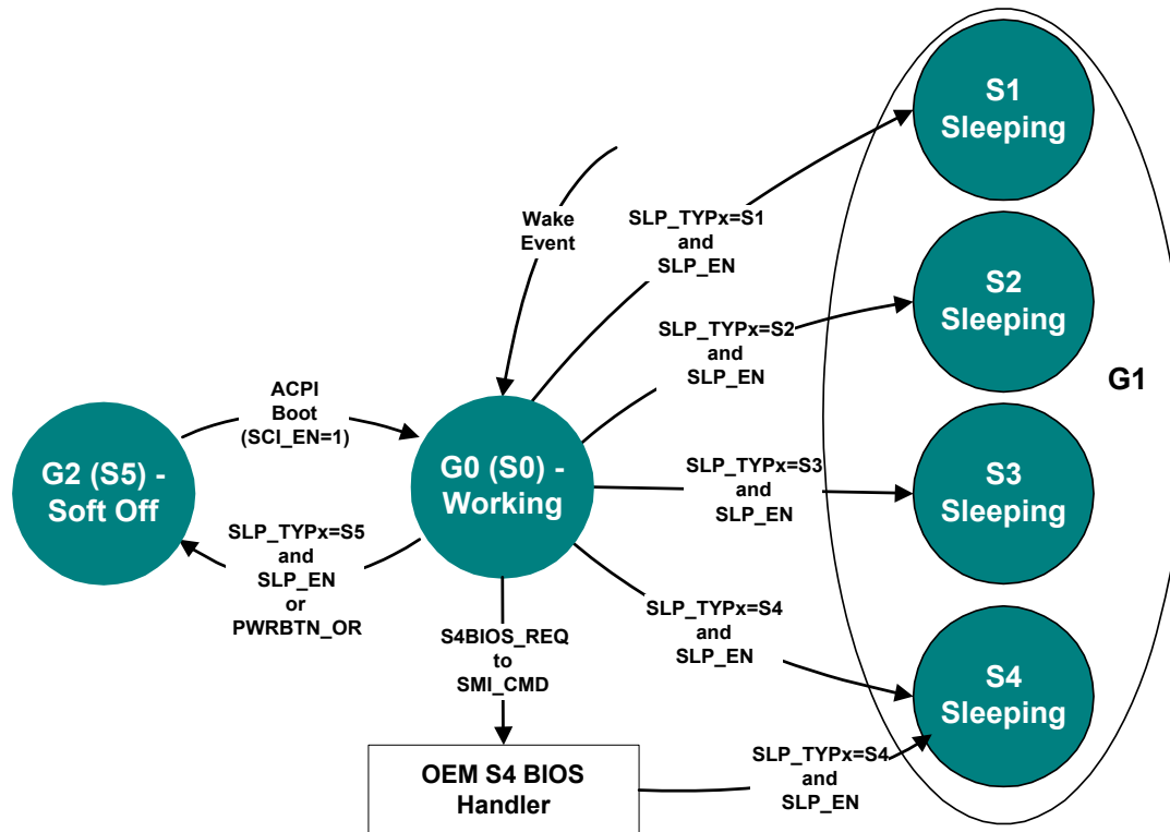
Figure 16-76 Example Sleeping States
