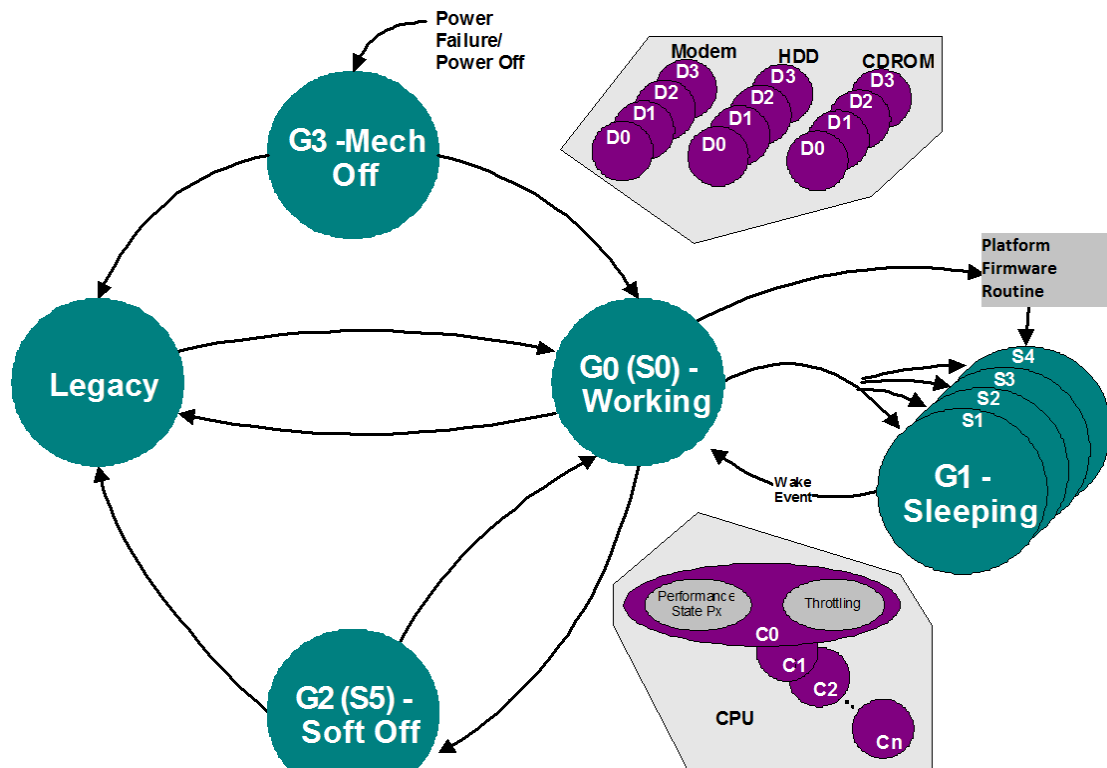
Figure 4-10 Global States and Their Transitions
