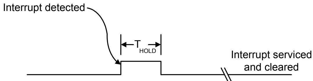
Figure 12-72 Interrupt Model
