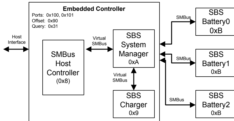
Figure 10-61 Smart Battery Subsystem
