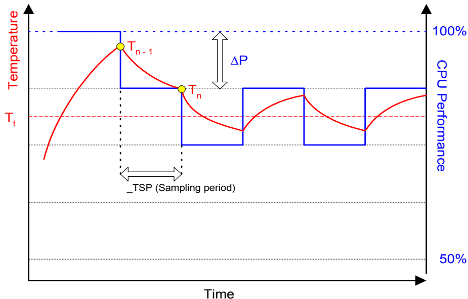
Figure 11-67 Temperature and CPU Performance Versus Time
