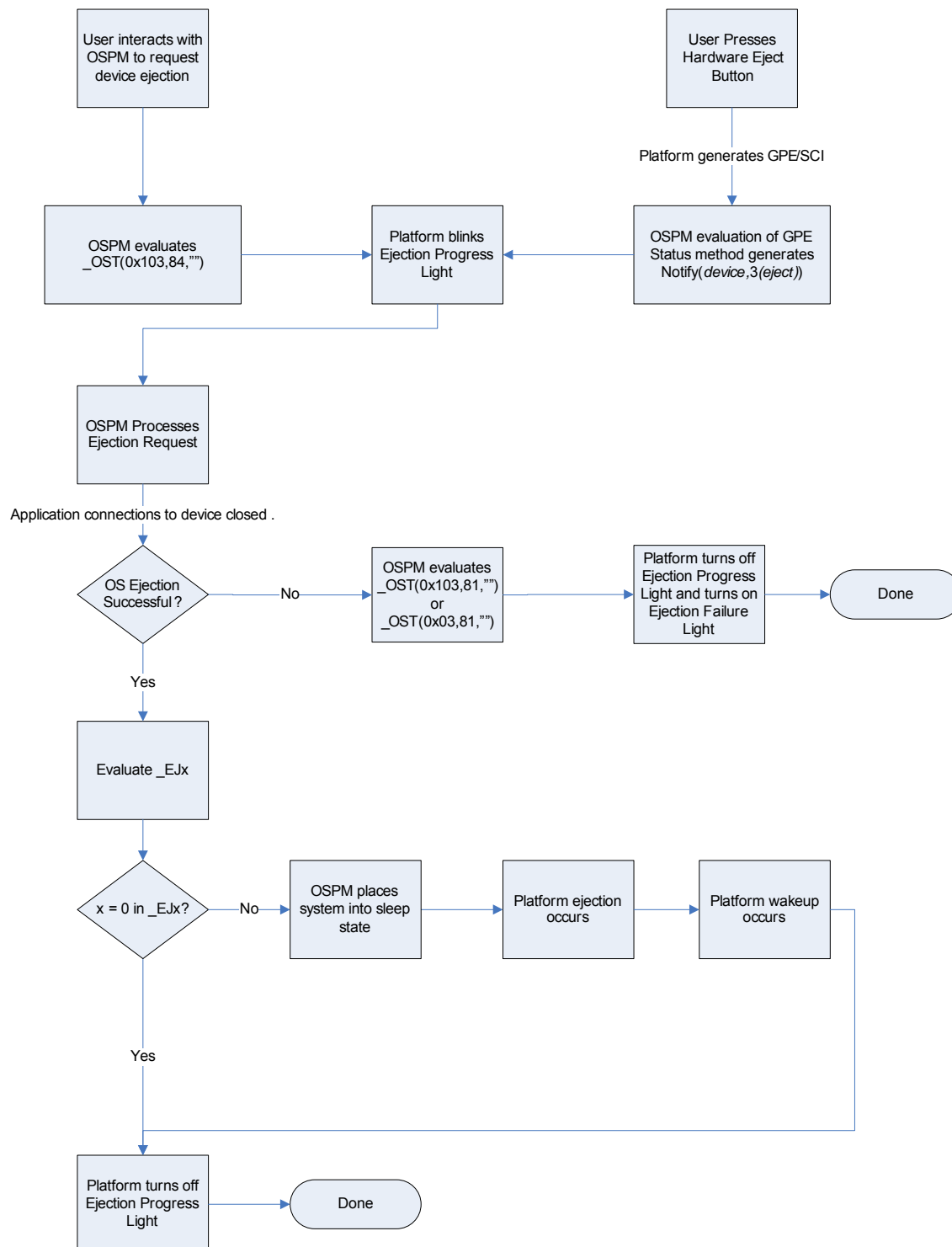
Figure 6-38 Device Ejection Flow Example Using _OST
