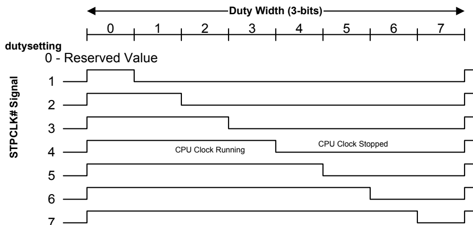
Figure 8-43 Example Control for the STPCLK#
