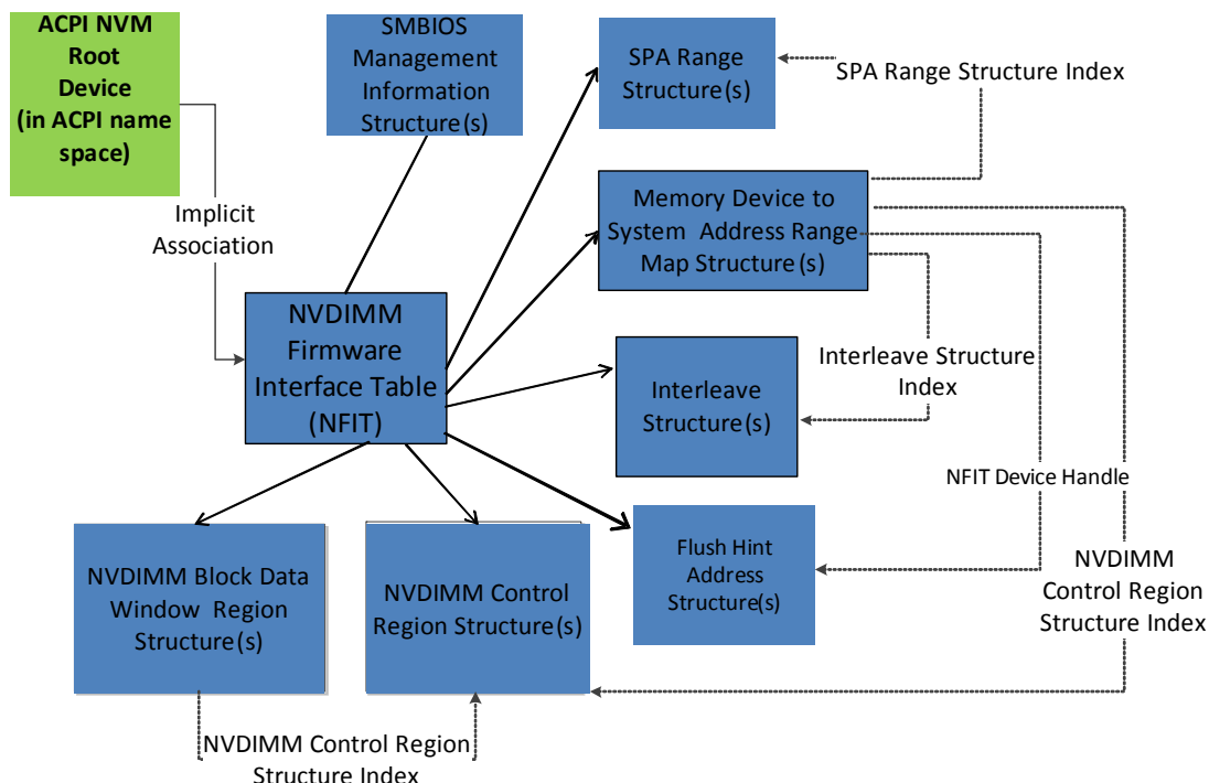
Figure 5-30 NVDIMM Firmware Interface Table Overview
