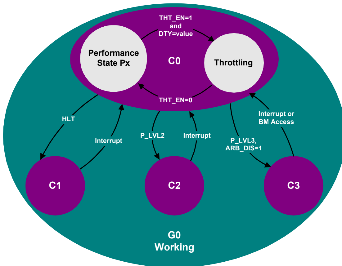
Figure 8-40 Processor Power States
