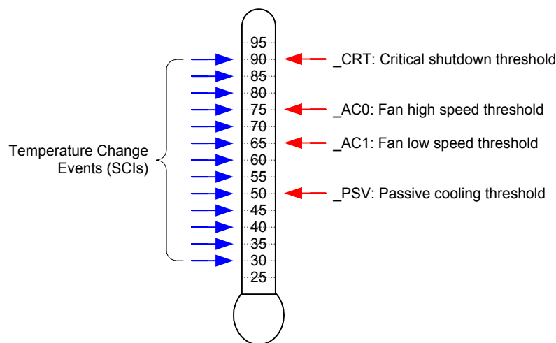
Figure 11-66 Thermal Events
