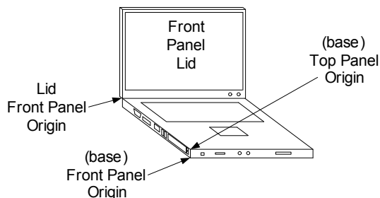
Figure 6-34 Laptop Panel and Panel Origin Positions
