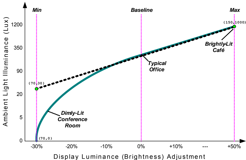
Figure 9-52 A two-point ALS Response Curve
