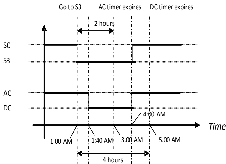
Figure 9-57 System transitions with WakeAlarm -- Policy
