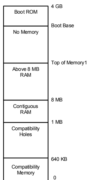
Figure 16-78 Example Physical Memory Map
