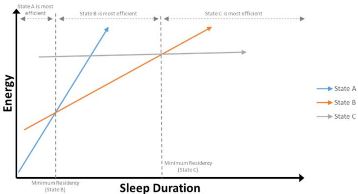
Figure 8-48 Energy of states A,B and C versus sleep duration
