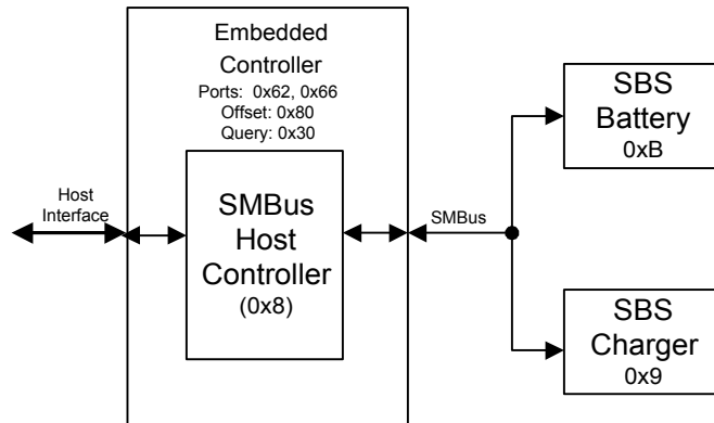
Figure 10-60 Single Smart Battery Subsystem
