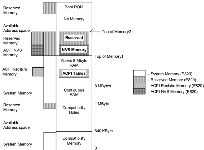
Figure 16-77 Memory as Configured after Boot
