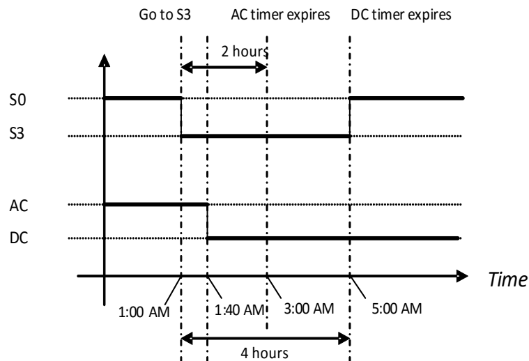
Figure 9-54 System transitions with WakeAlarm -- Timer
