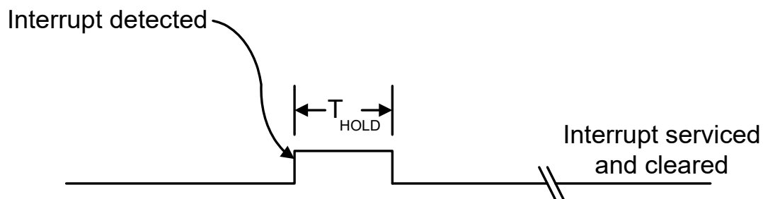
Figure 12-70 Interrupt Model
