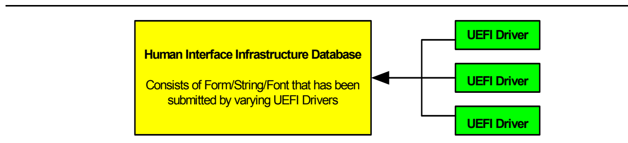
Figure 103. HII Database
