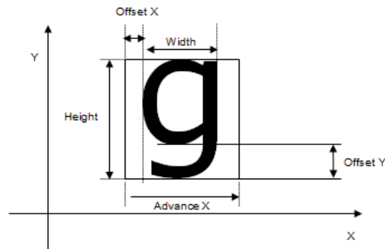
Figure 130. Glyph Example
