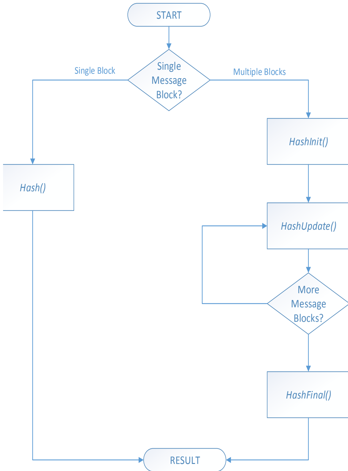
Figure 134. Hash workflow
