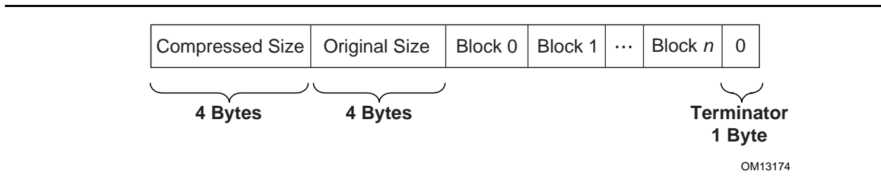
Figure 57. Compressed Data Structure
