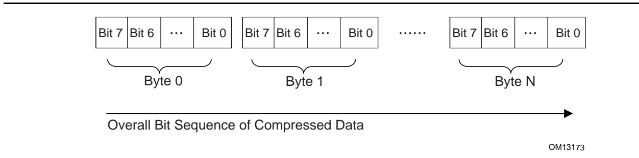
Figure 56. Bit Sequence of Compressed Data
