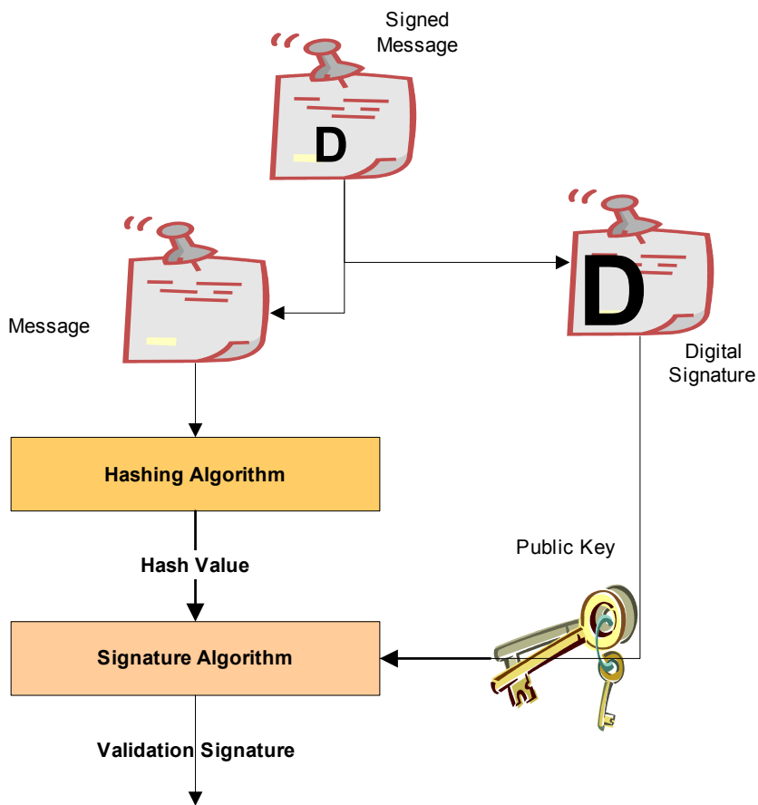
Figure 75. Verifying a Digital Signature
