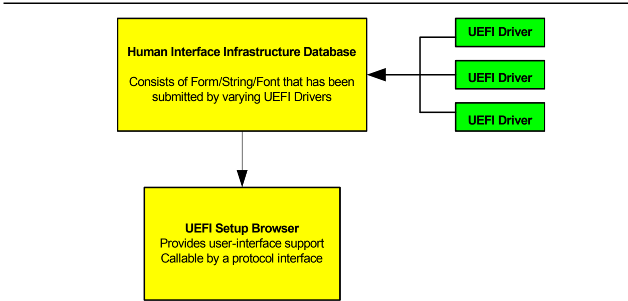
Figure 104. Setup Browser
