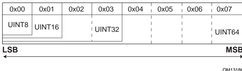
Figure 142. Storage Types
