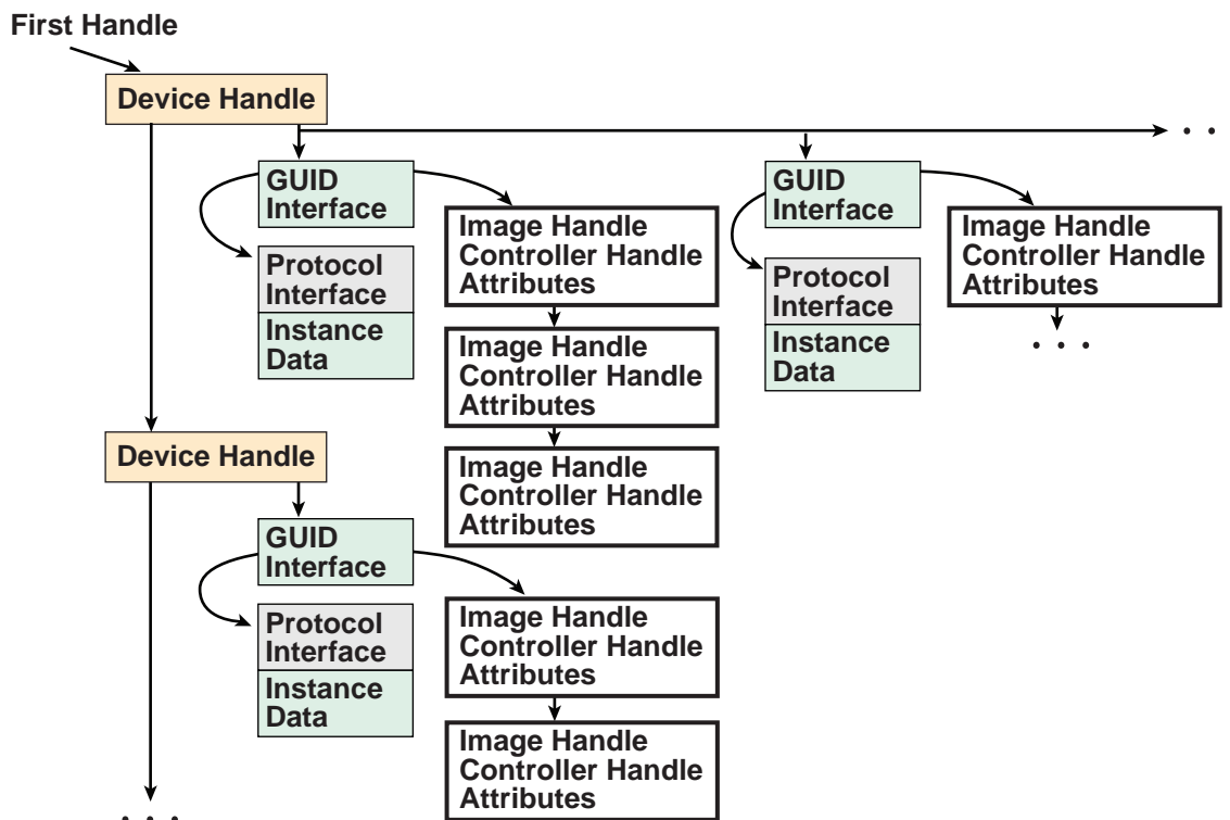
Figure 21. Handle Database
