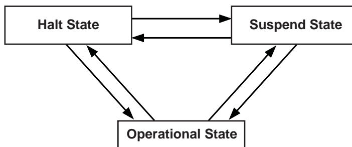
Figure 48. Software Triggered State Transitions of a USB Host Controller
