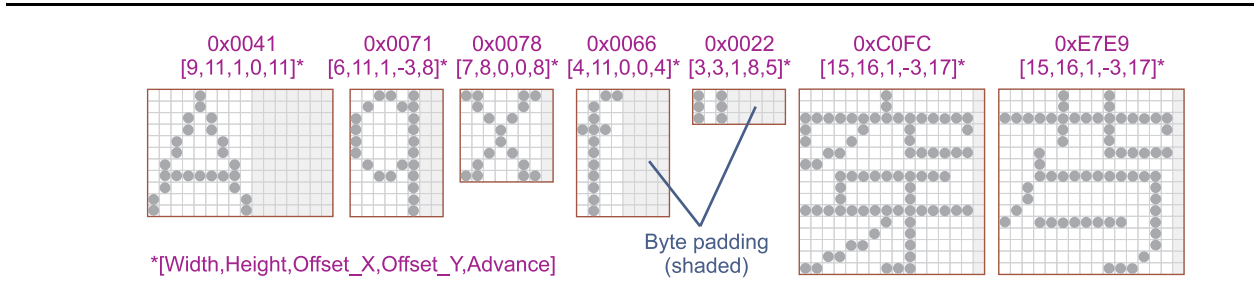
Figure 87. Proportional Font Parameters and Byte Padding
